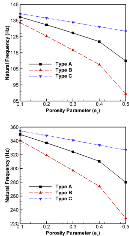
Figure 3: Variation of the natural frequency of clamped folded plates in relation to porosity parameters across various porous distributions, a) n=1 and b) n=2 ( L_1 = L_2 = 0.5m, b = 0.2m, h = 1mm, m = 1 )
